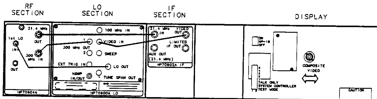
Figure 2-3. Typical HP 71100A Spectrum Analyzer Rear-Panel Cables
