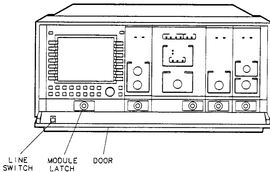
Figure 2-2. Module Installation
