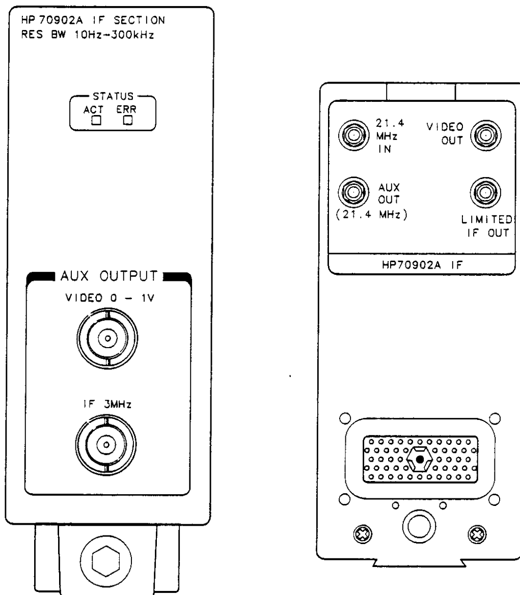
Figure 1-2. Module Front- and Rear-Panel Features
